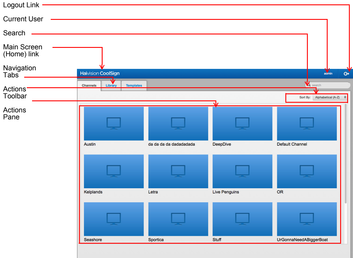
Figure 4 Interface Screen Elements
